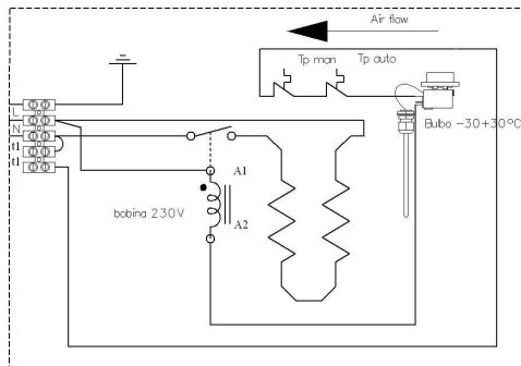
REF-FL-SCTTC single phase With contactor and adjustable automatic reset thermostat 0-90°C
