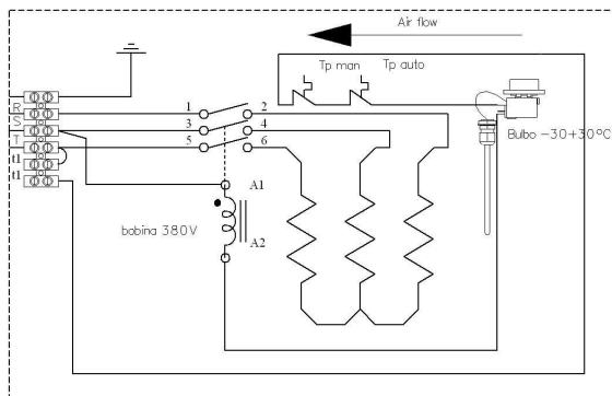
REF-FL-SCTTC three phases With contactor and adjustable automatic reset thermostat 0-90°C
